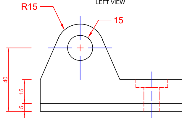
LEFT VIEW
