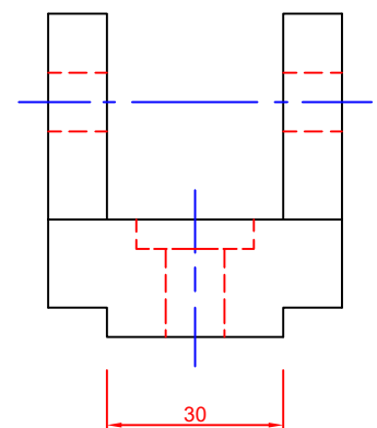
FONT VIEW
