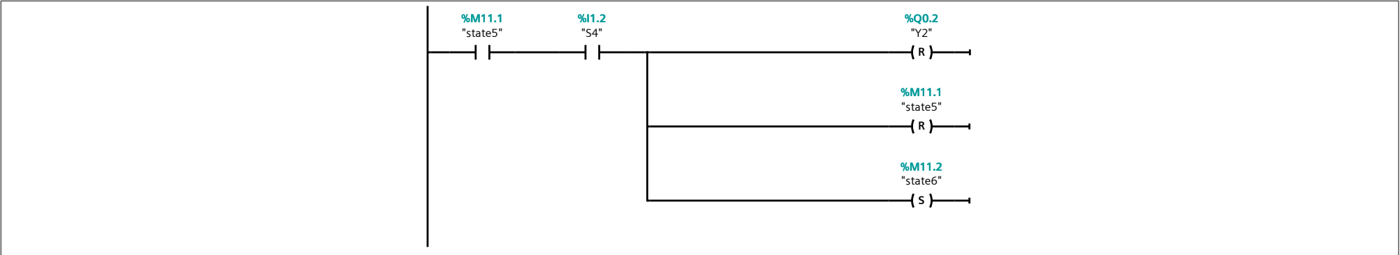
Network 12: Start command
