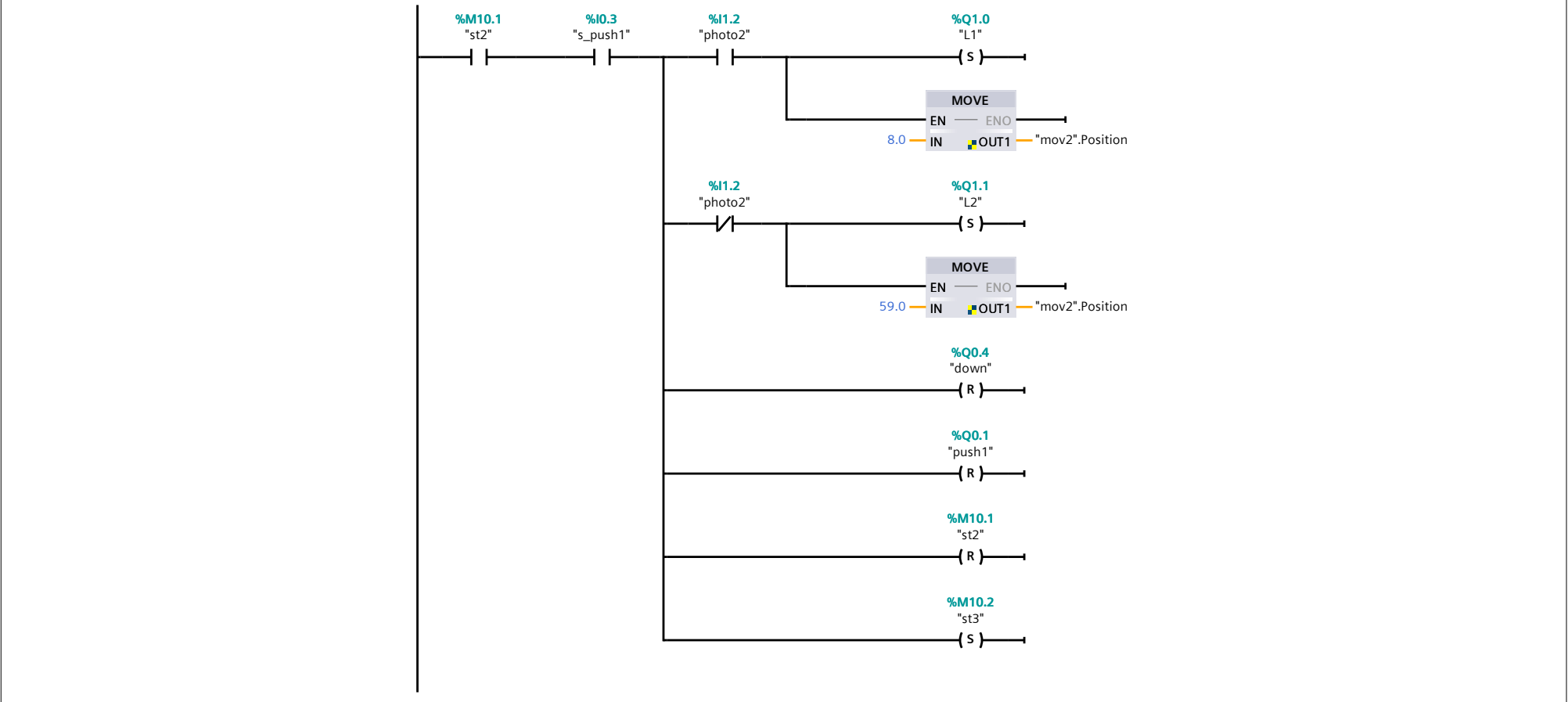
Network 6: Start command
