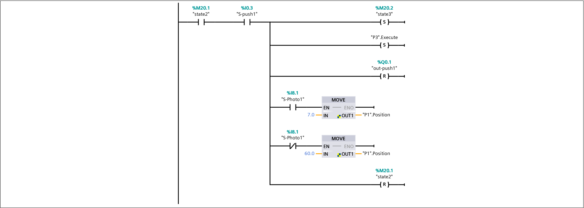
Network 7:
