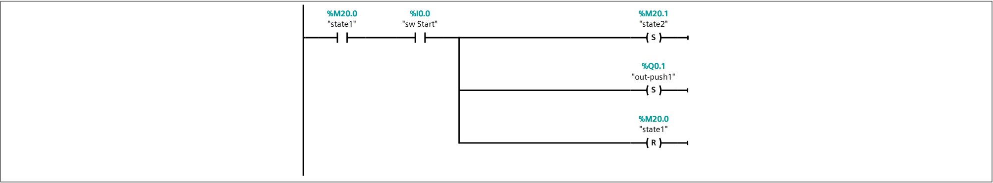
Network 6:
