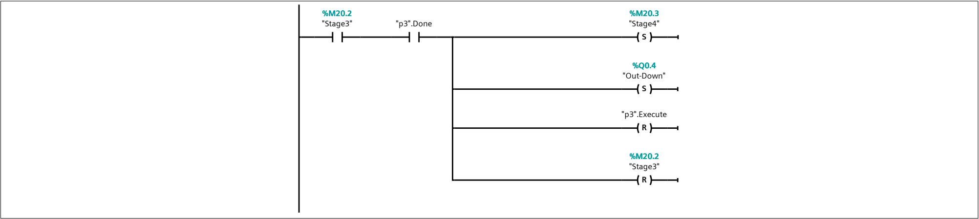
Network 8: Start command
