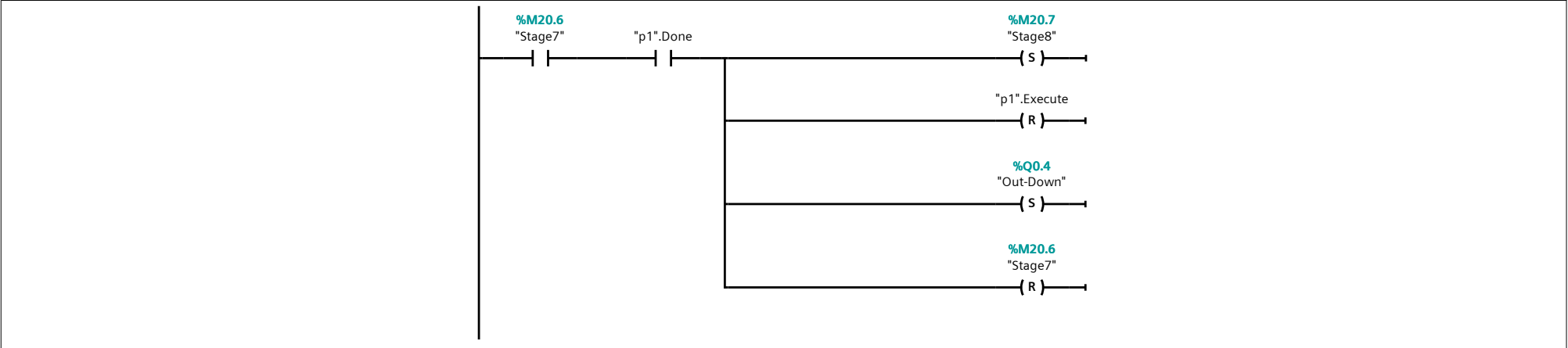
Network 12: Start command
