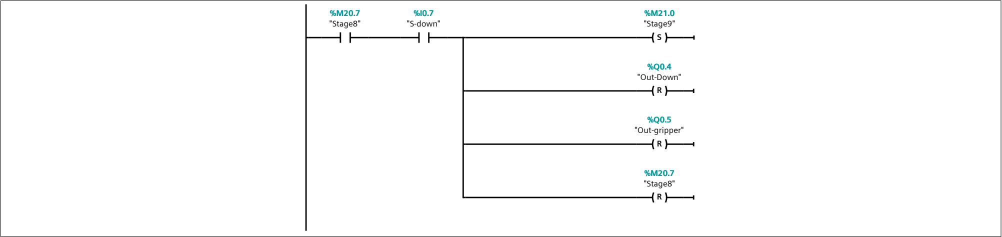
Network 13: Start command
