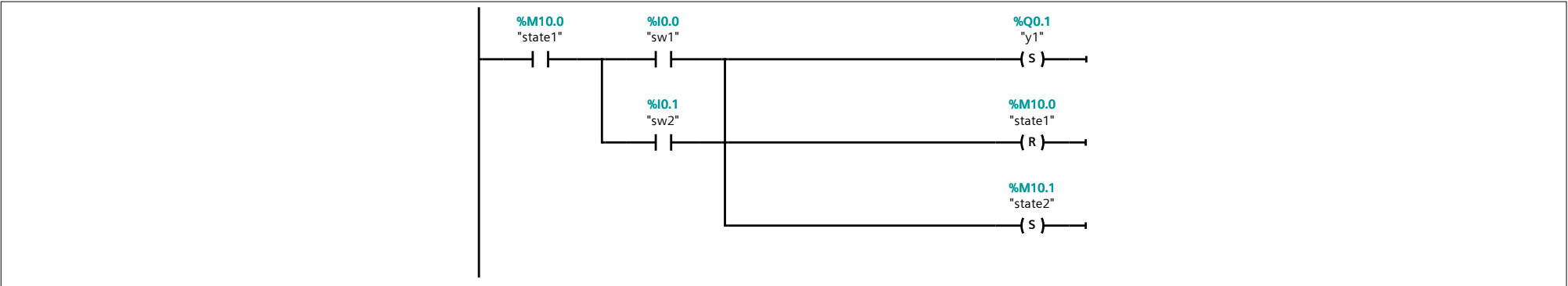
Network 7: Start command
