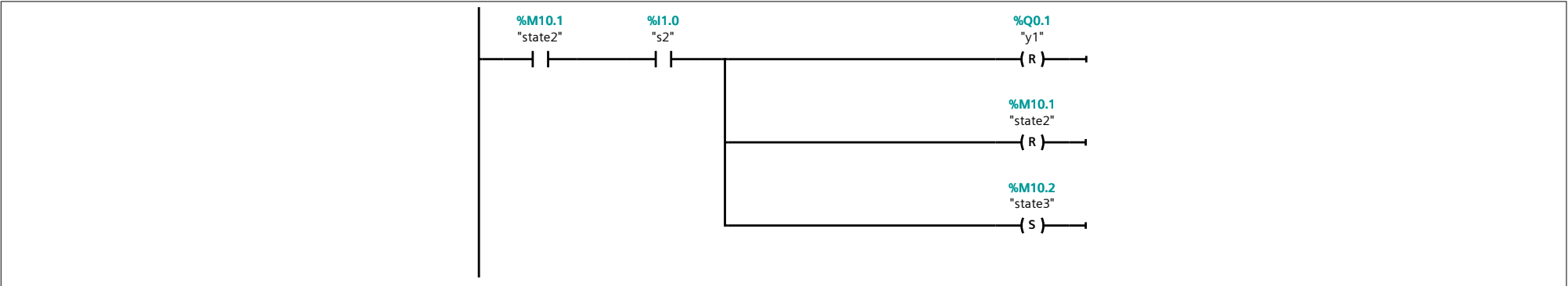
Network 8: Start command
