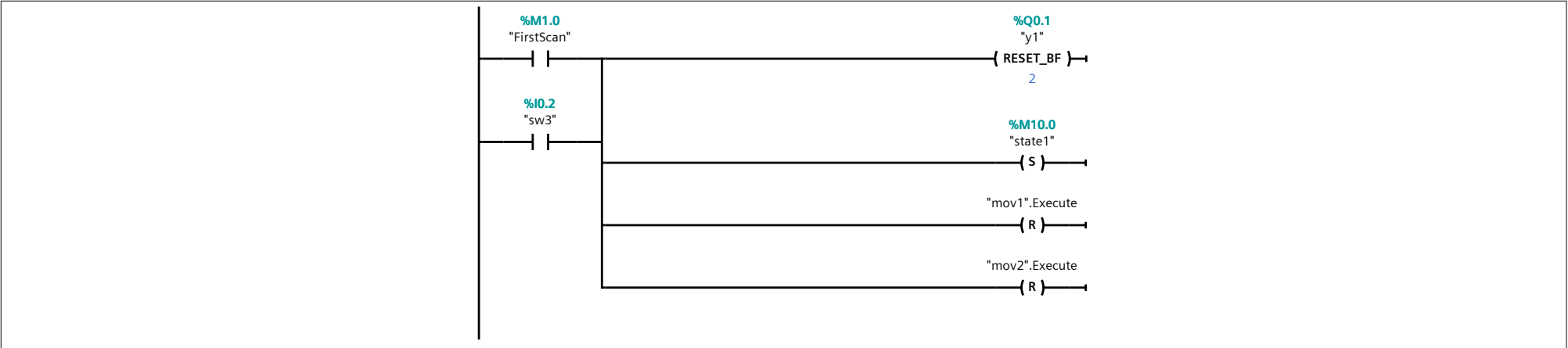
Network 6: Start command
