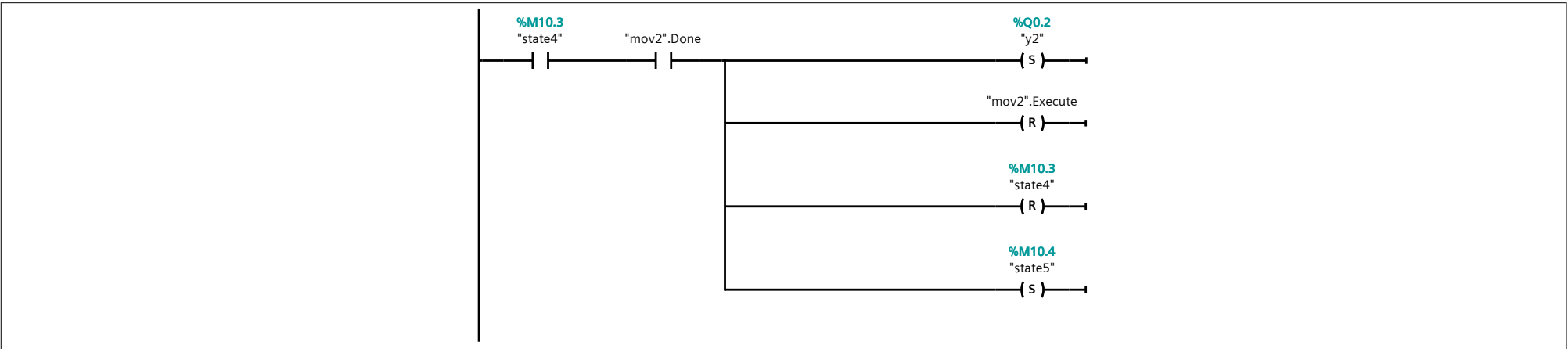
Network 10: Start command
