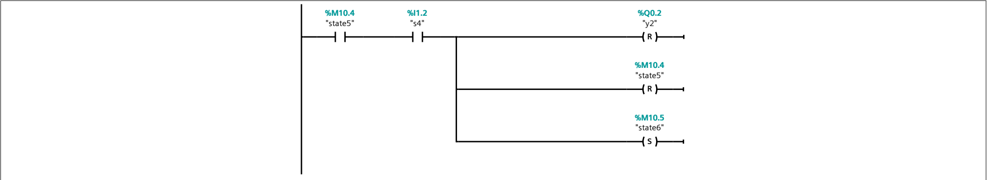
Network 11: Job is completed
