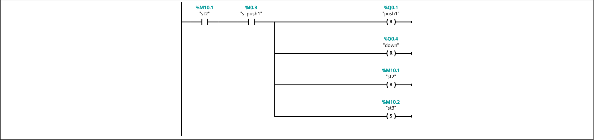
Network 9: Start command
