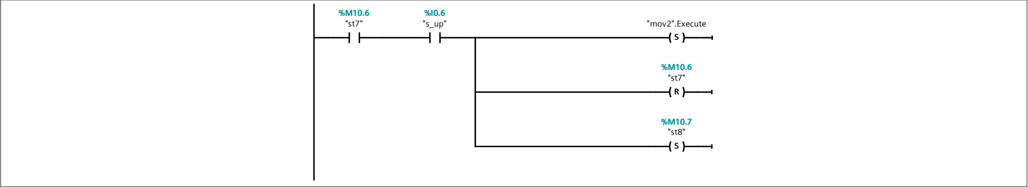
Network 14: Start command
