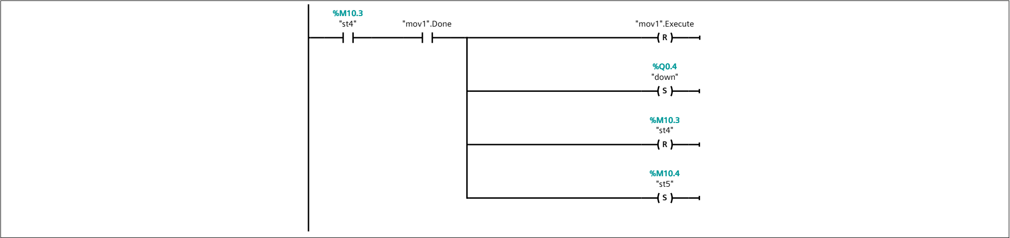
Network 11: Start command
