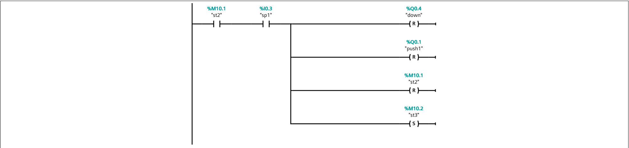
Network 8: Start command
